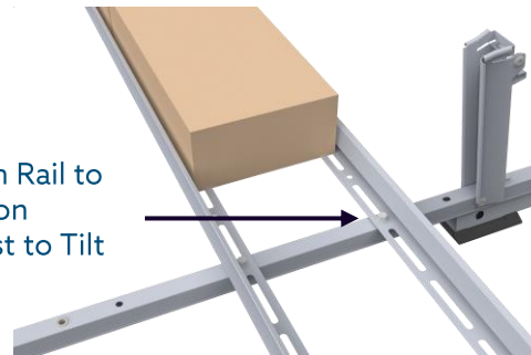
Rail Position for Ballast blocks
