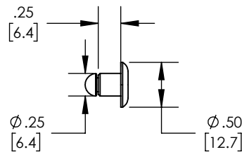
3) RIVET, 1/4"x .25"L, .020-.125 GRIP, ST
