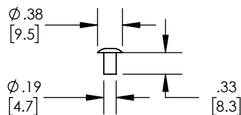
3) RIVET, 3/16", .020-.125 GRIP, ST
