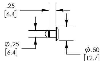
4) RIVET, 1/4"x .25"L, .020-.125 GRIP, ST
